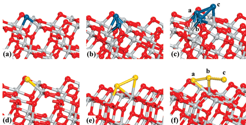
Figure 5. Calculated structures of adsorbed Pt/Au (a)/(d) monomer, (b)/(e) dimer, and (c)/(f) trimer at the O vacancy of anatase TiO 2 (101) terraces.
