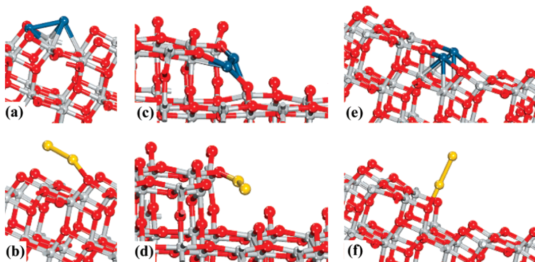
Figure 3. Calculated structures of adsorbed Pt/Au dimers at (a)/(b) terraces, (c)/(d) step D-(112), and (e)/(f) step B-(100) of anatase TiO 2 (101) surfaces.
